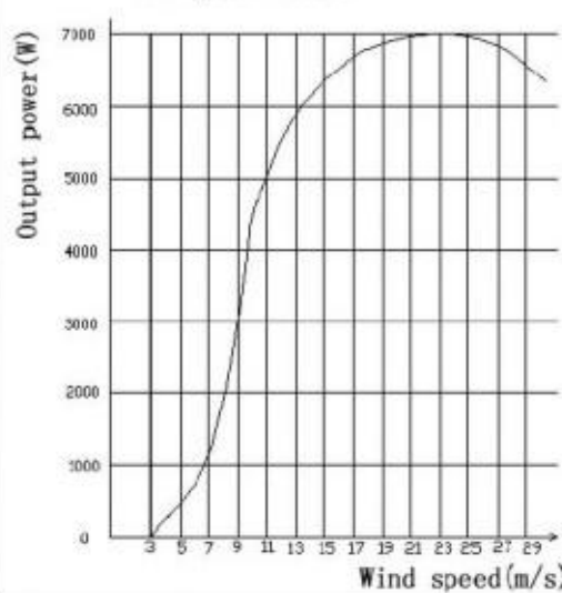
5KW power curve
